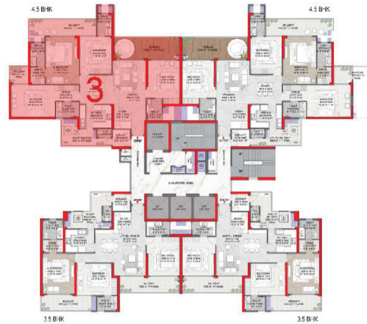
CLUSTER PLAN
